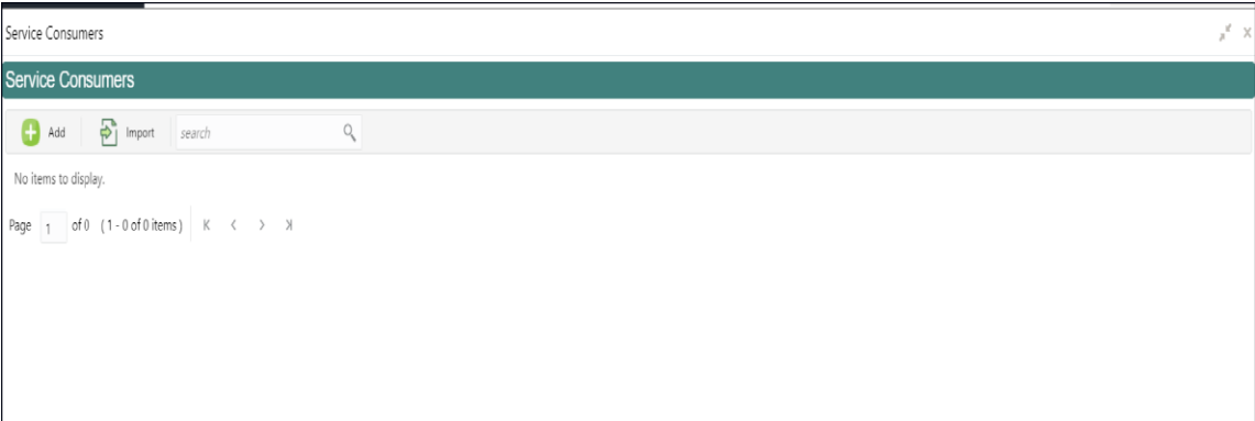
Figure 5: Service Consumers
